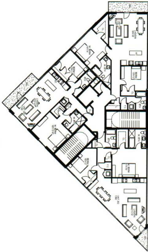
② SECOND FLOOR PLAN
